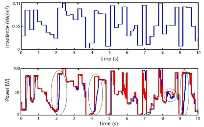
Fig. 17. Maximum Power Point Tracking under fixed temperature (25°C) and random irradiance input: traditional Perturb and Observe algorithm (blue curve), developed Fuzzy Logic–Perturb and Observe algorithm (red curve).
