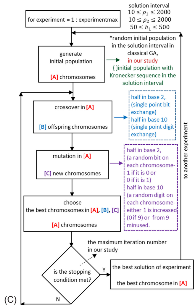
Fig. 2. (A) crossover, (B) mutation, (C) genetic algorithm running scheme.
