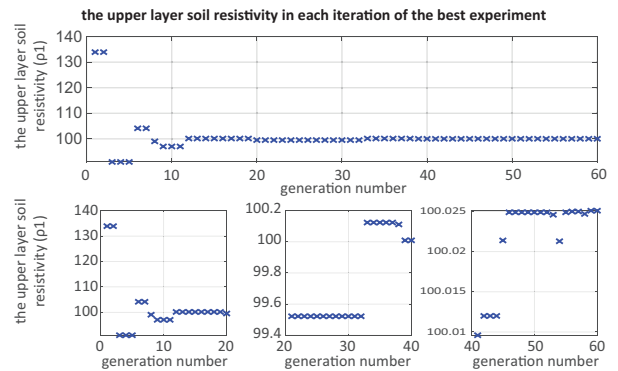
(B) The upper layer soil resistivity in the best experiment
