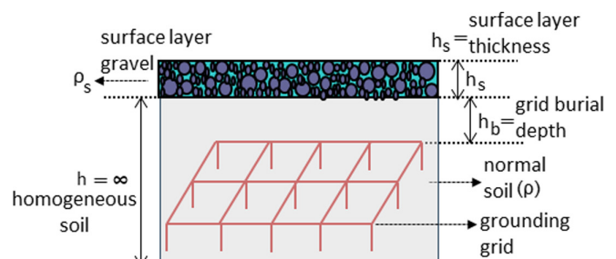
Fig. 4. Uniform soil model.
