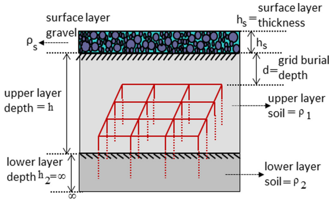
Fig. 5. Two-layer soil model.
