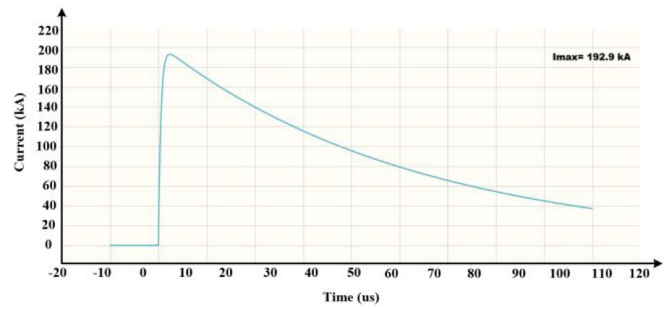
Fig. 6. Output signal of the high current generator using a copper connector with a diameter of 1 mm.
